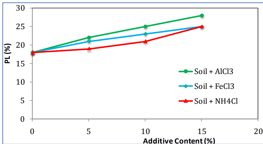
Fig. 2. Influence of AlCl 3 , FeCl 3 , and NH 4 Cl on plastic limit
