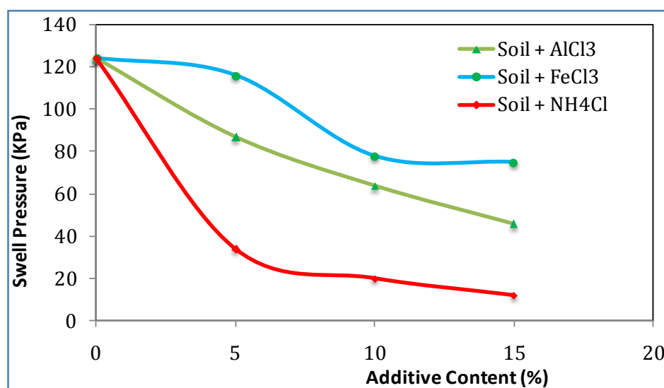
Fig. 5. Variation of swell pressure with various AlCl 3 , FeCl 3 , and NH 4 Cl contents
