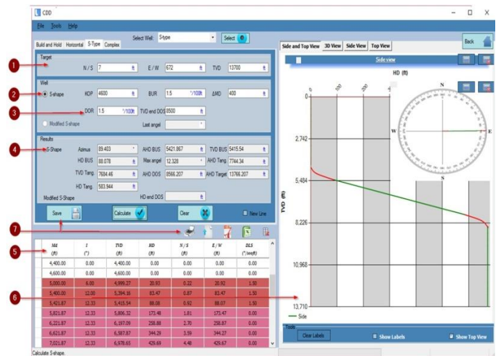
Fig. 4. CDD Well Mode main sections
