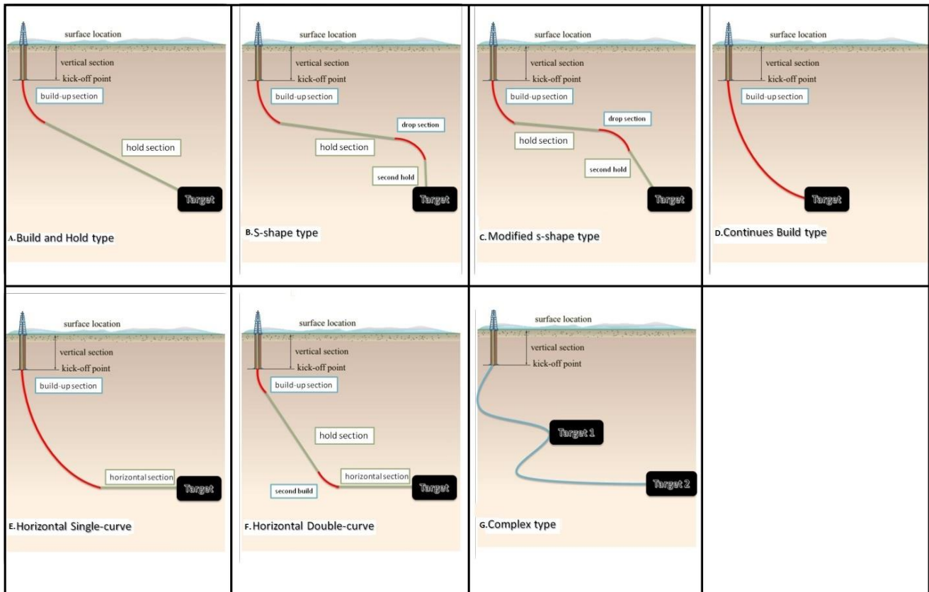
Fig. 1. Directional Drilling well types
