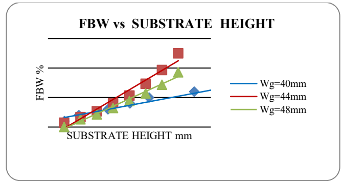
Fig. 2. (b) FBW vs. Substrate Height (Various W_g values)
