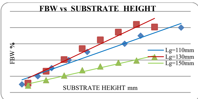
Fig. 2. (a) FBW vs. Substrate Height (Various L_g values)
