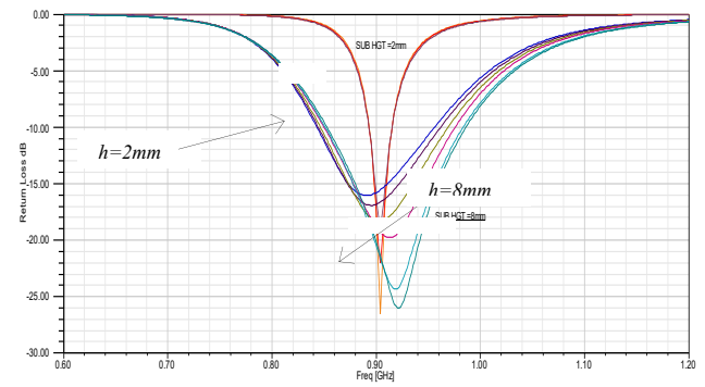
Fig .6. Effect of the Feed Position
