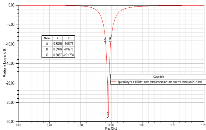
Fig .8. Return Loss
