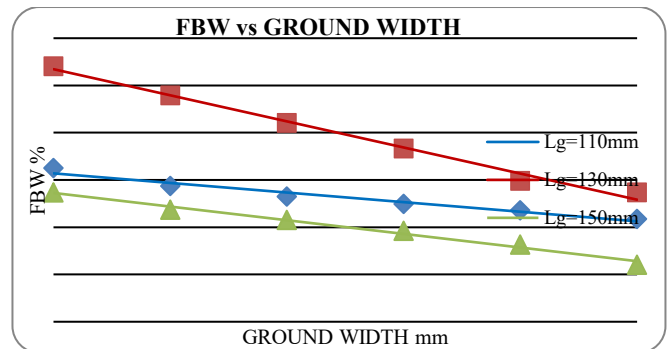
Fig. 3. (b) FBW vs. Ground Width (Various L_g values)
