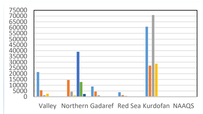
Fig .4. Average concentrations of particulate matter 10 micron in all states under study.
