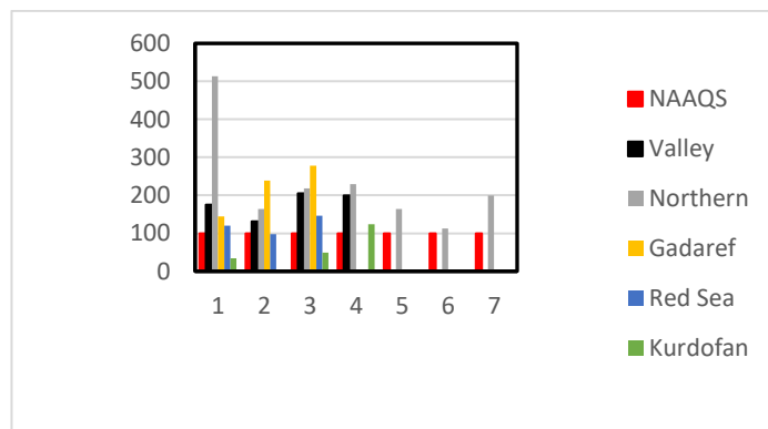
Fig .5. Average concentrations of nitrogen dioxide in all locations.
