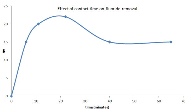
Fig. 1. Effect of contact time on fluoride removal [Source Mwangi C. et al. (2016)].
