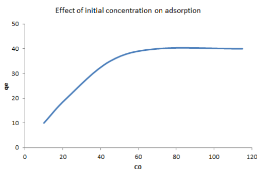
Fig. 2. Effect of initial fluoride concentrations on fluoride removal. [Source: Kamathi Mwangi C. et al., (2016)].
